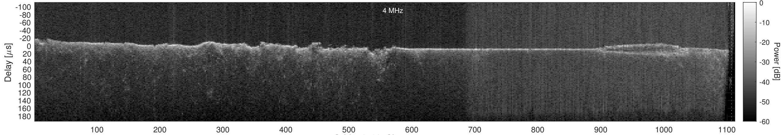
Orbit 12102, Cluttergram
