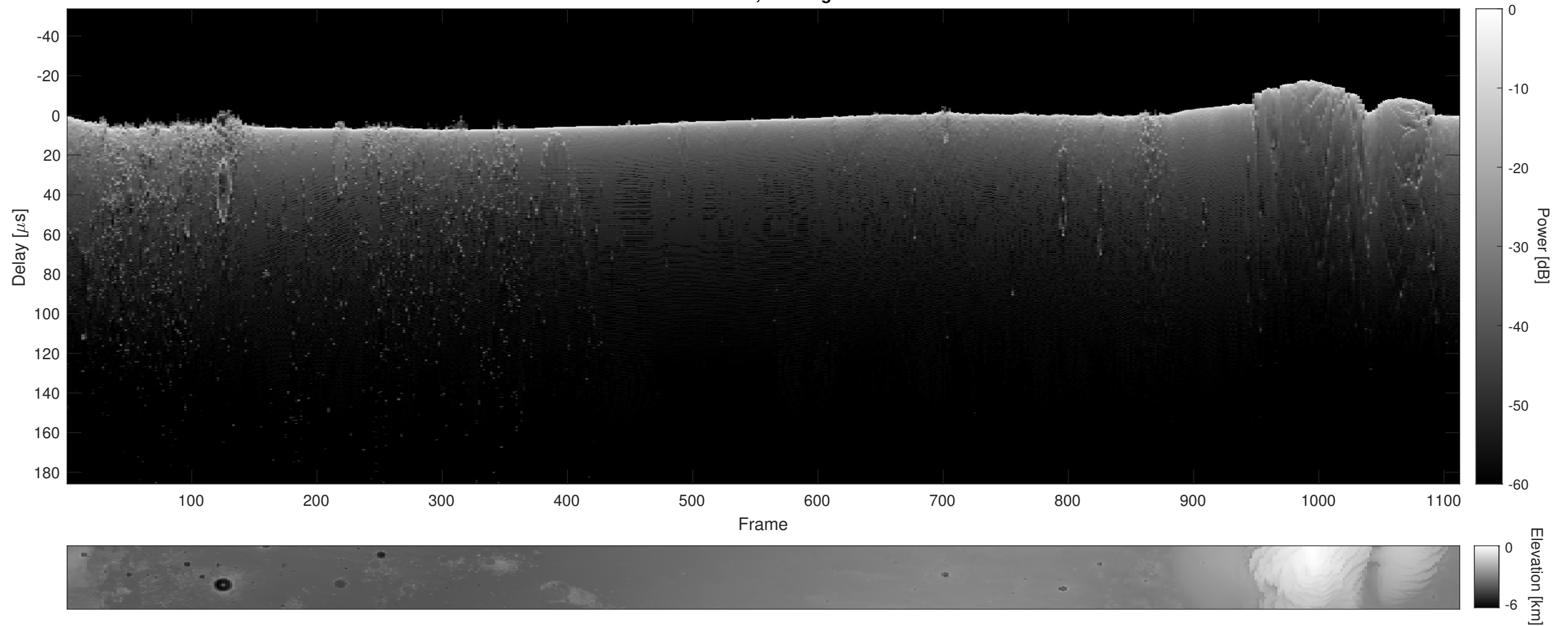
Orbit 12104, Cluttergram
