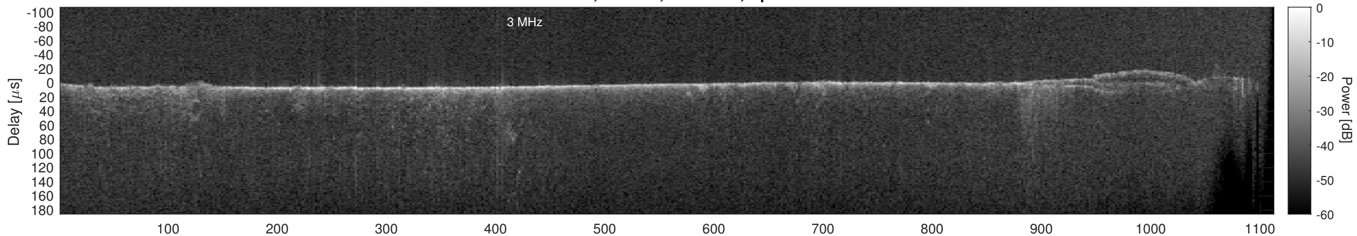
Orbit 12104, Cluttergram
