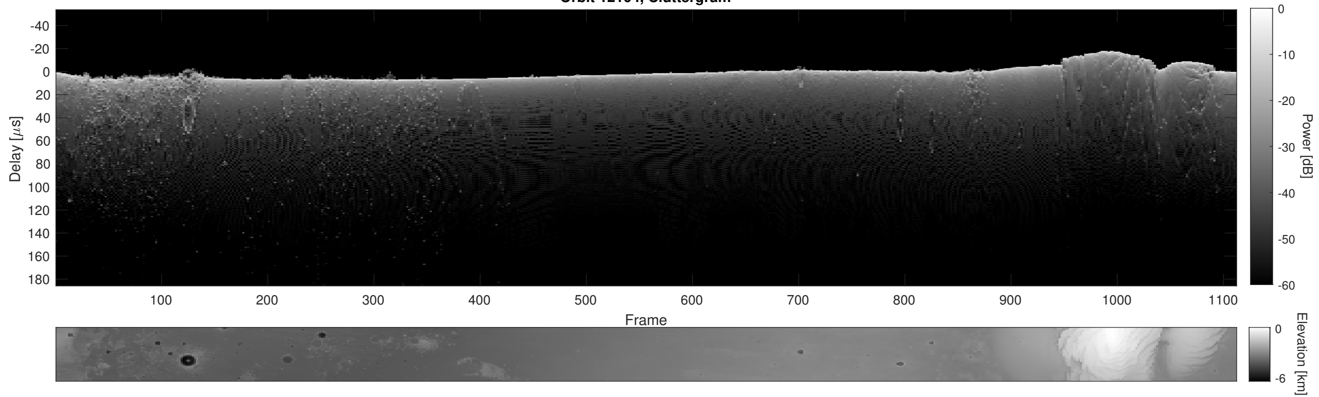
Orbit 12104, Cluttergram
