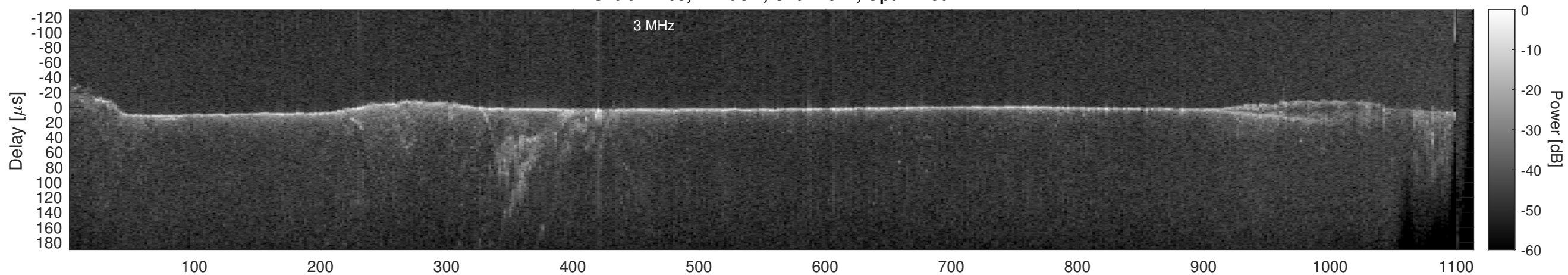
Orbit 12105, Cluttergram
