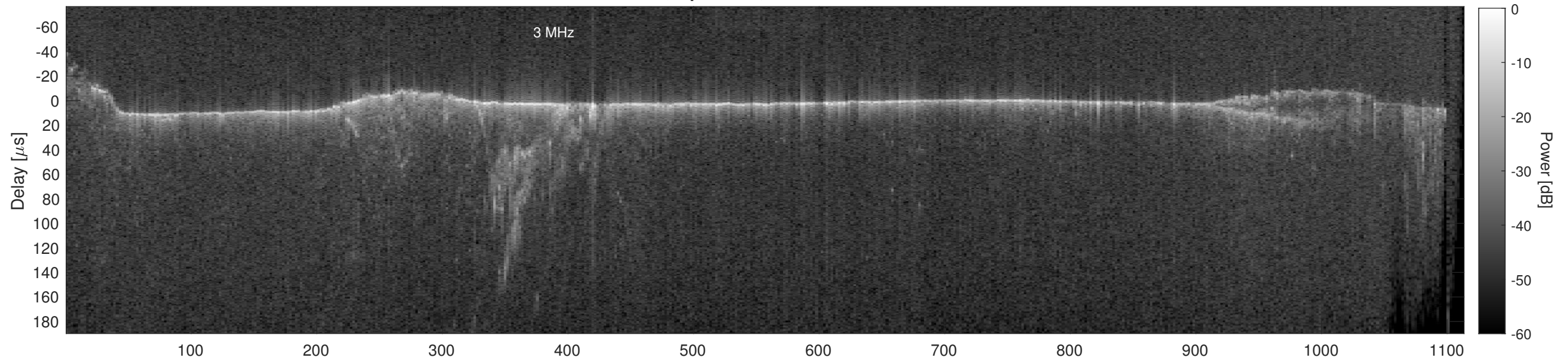
Orbit 12105, Cluttergram
