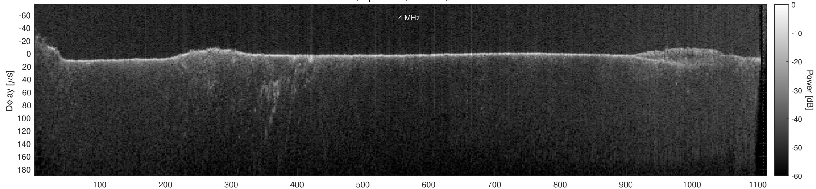
Orbit 12105, Optimized, Window, Channel 2
