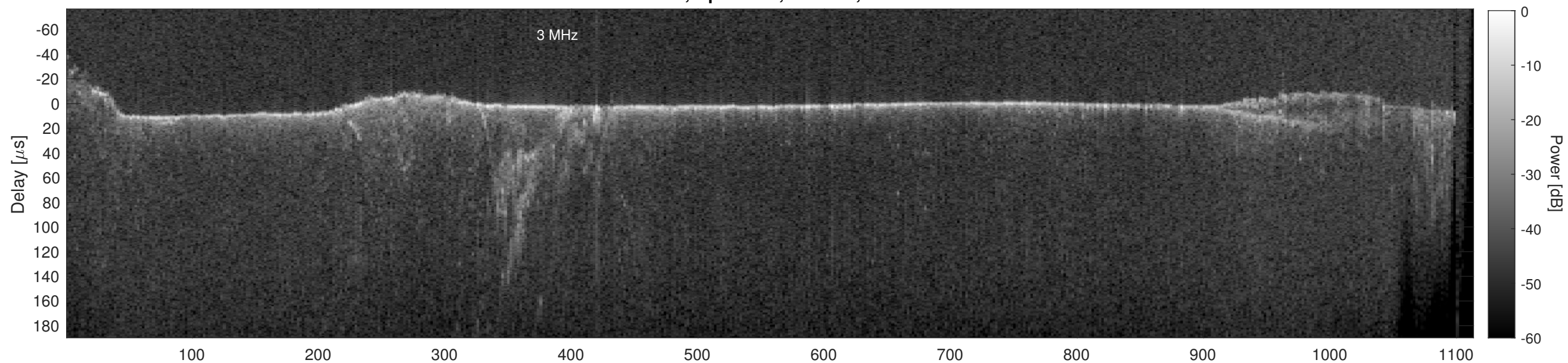
Orbit 12105, Cluttergram
