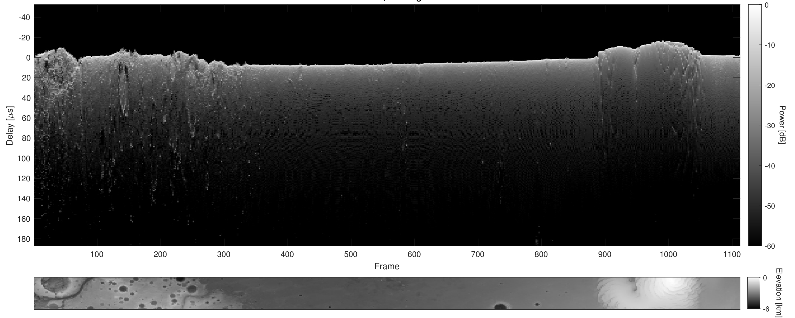
Orbit 12106, Cluttergram
