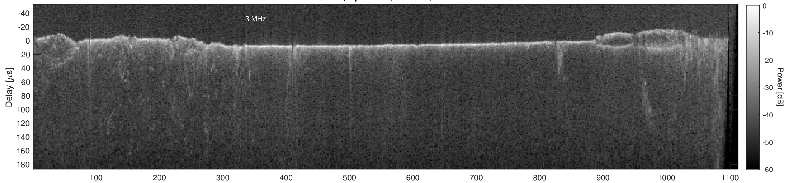
Orbit 12106, Cluttergram
