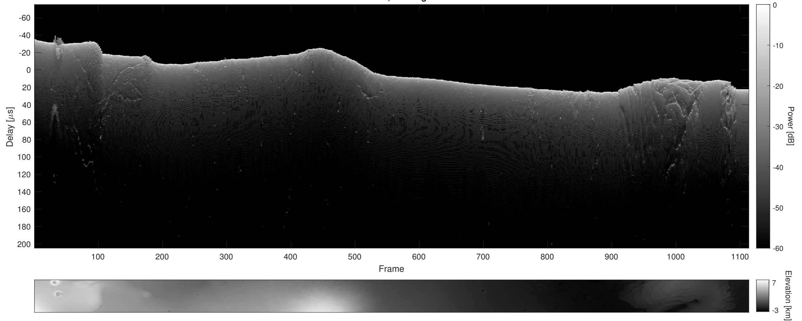
Orbit 12107, Cluttergram
