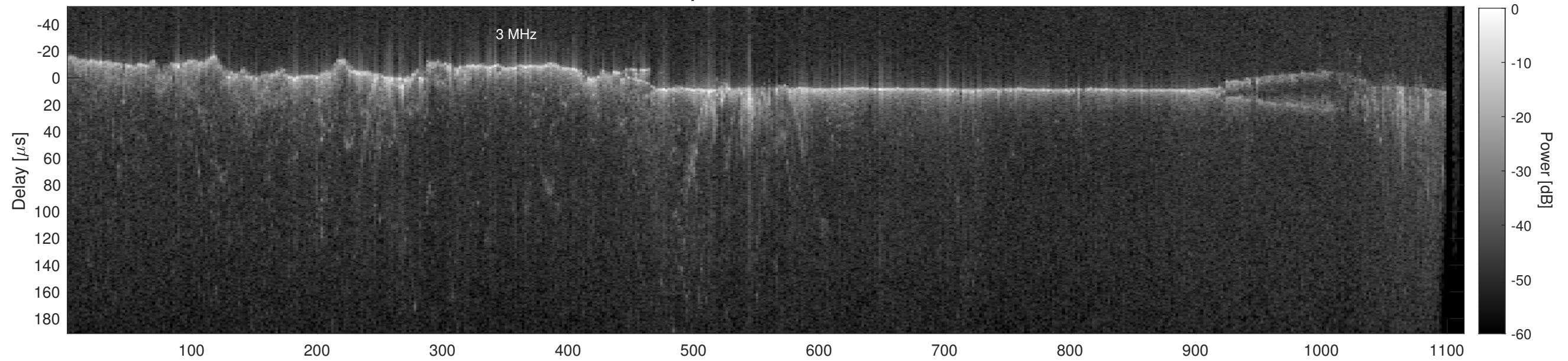
Orbit 12109, Cluttergram
