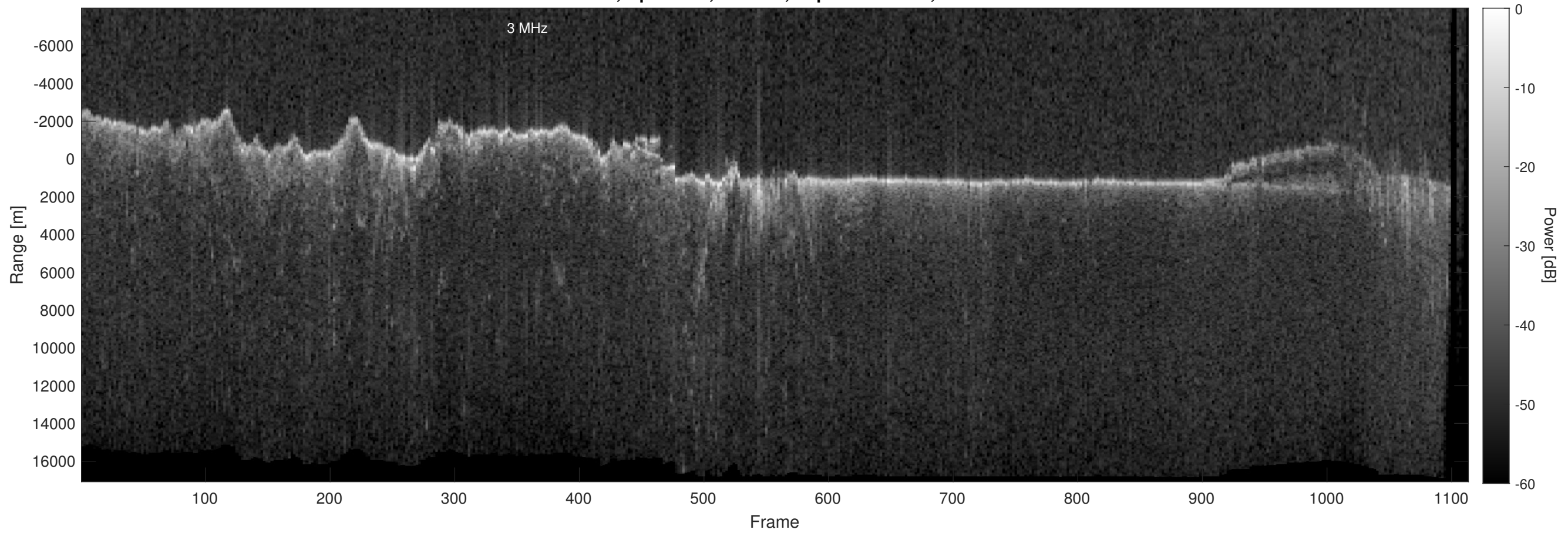
Orbit 12109, Optimized, Window, Depth-Corrected, Channel 2
