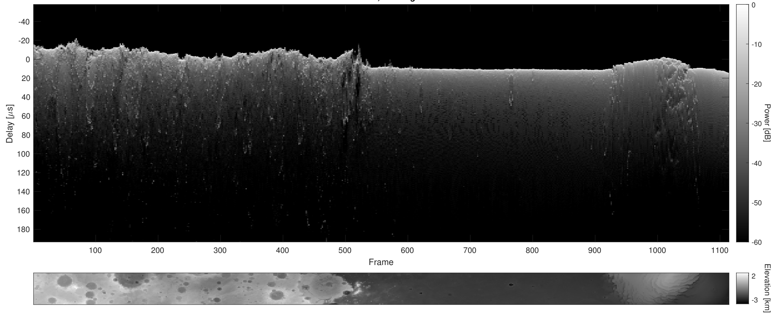
Orbit 12116, Cluttergram
