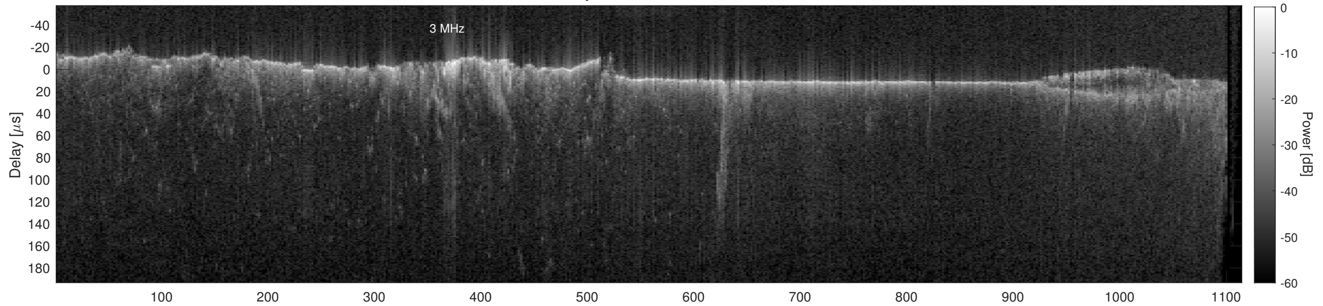
Orbit 12116, Cluttergram
