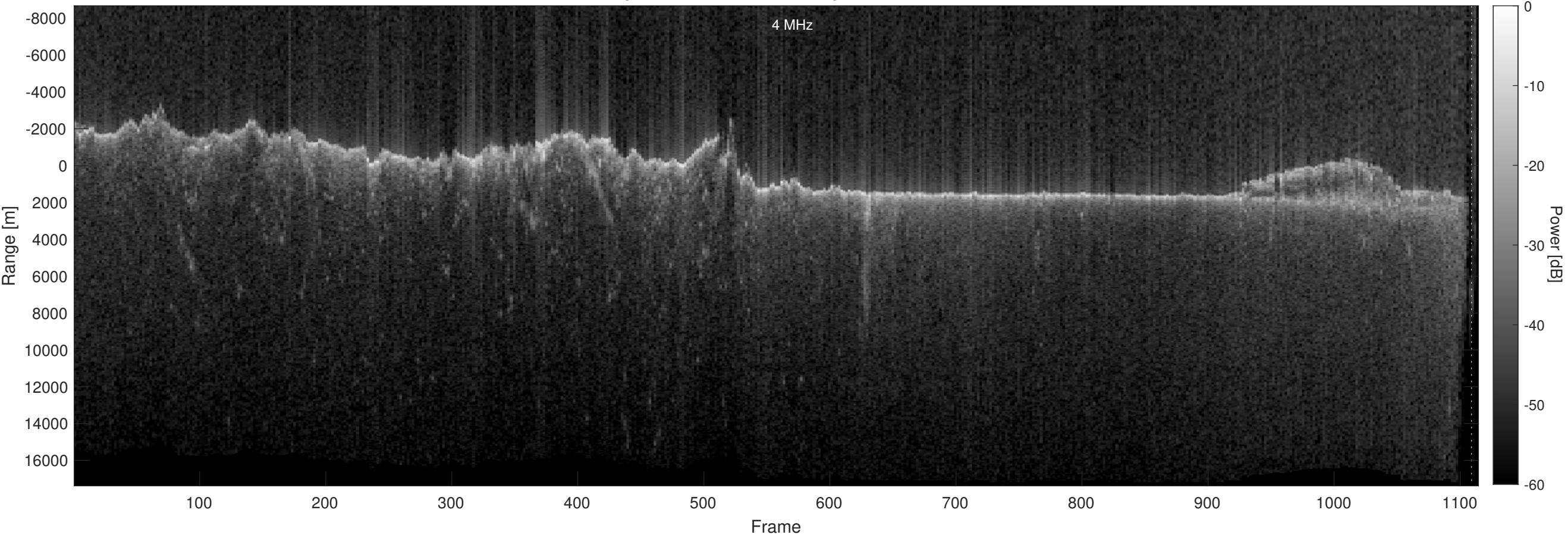
Orbit 12116, Optimized, No Window, Depth-Corrected, Channel 2
