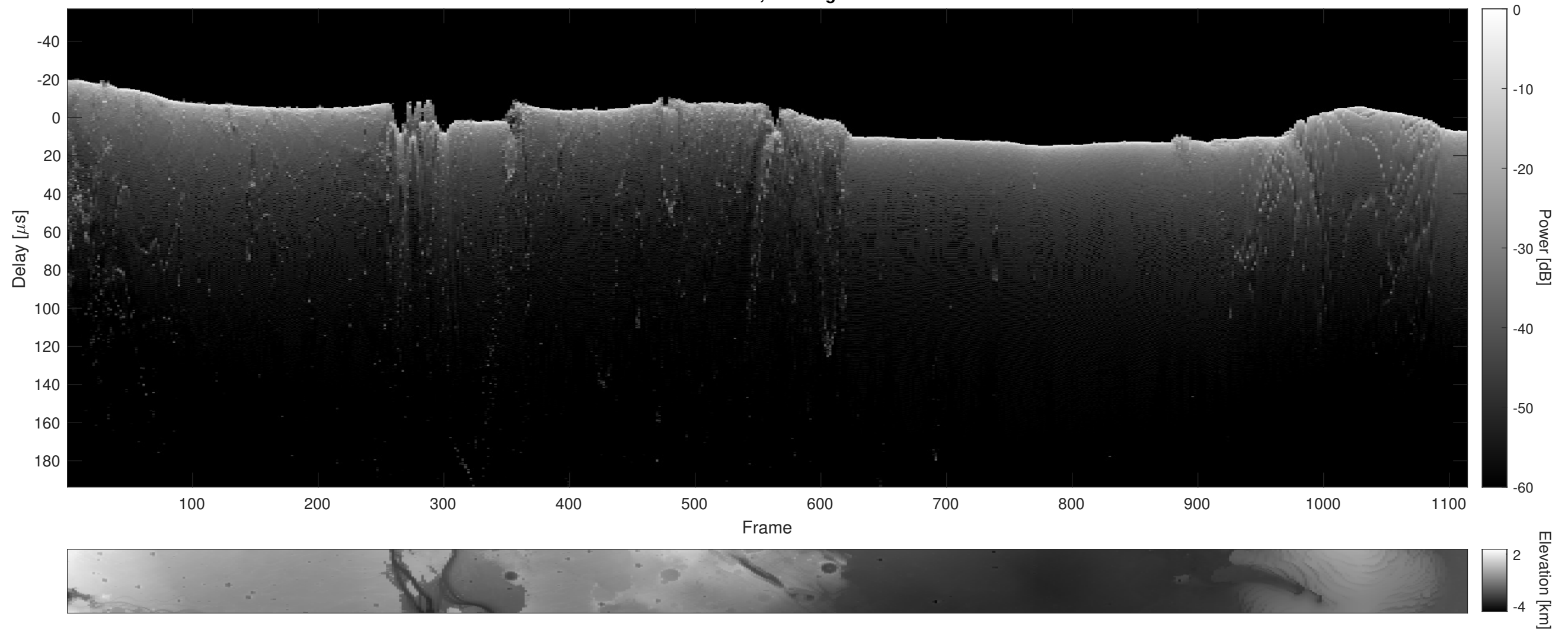
Orbit 12117, Cluttergram
