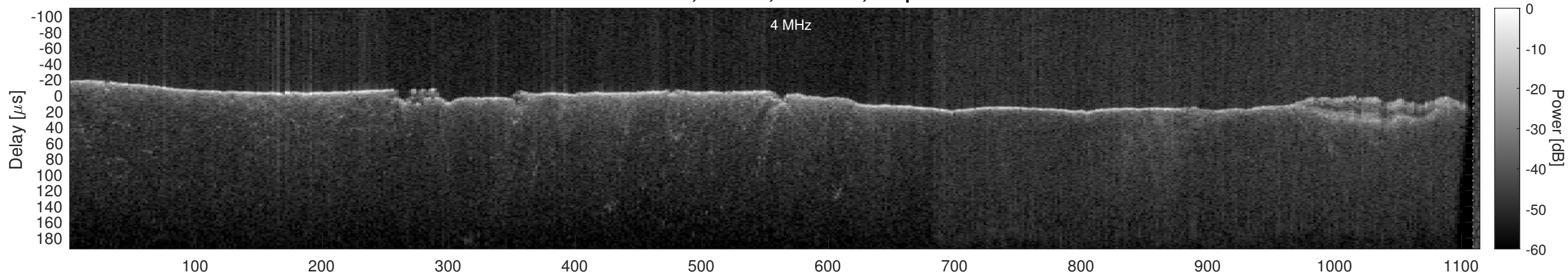
Orbit 12117, Window, Channel 1, Optimized
