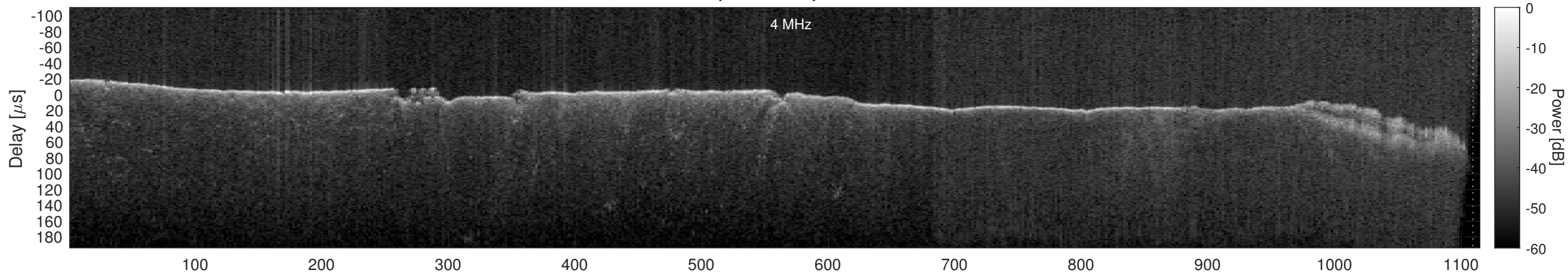
Orbit 12117, Window, Channel 1, Chapman
