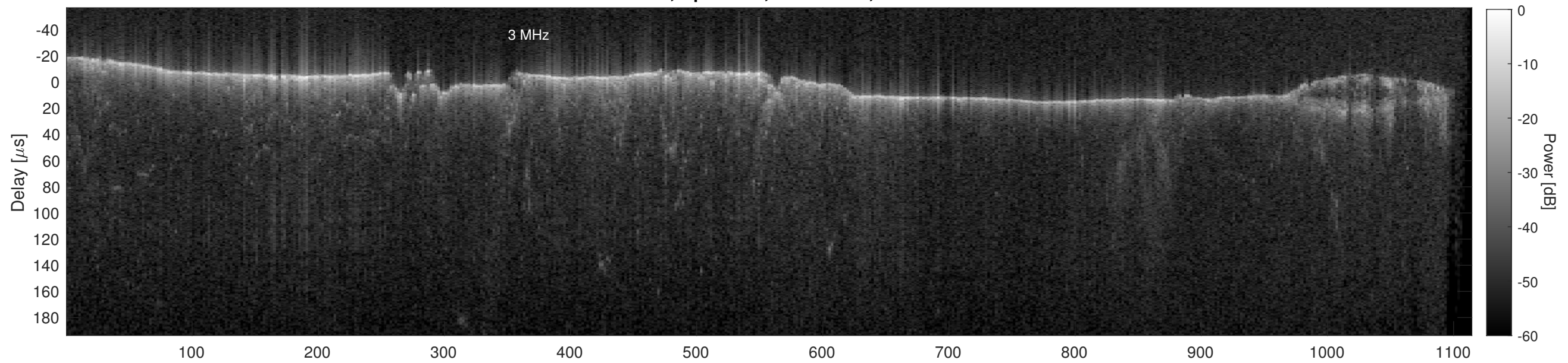
Orbit 12117, Cluttergram
