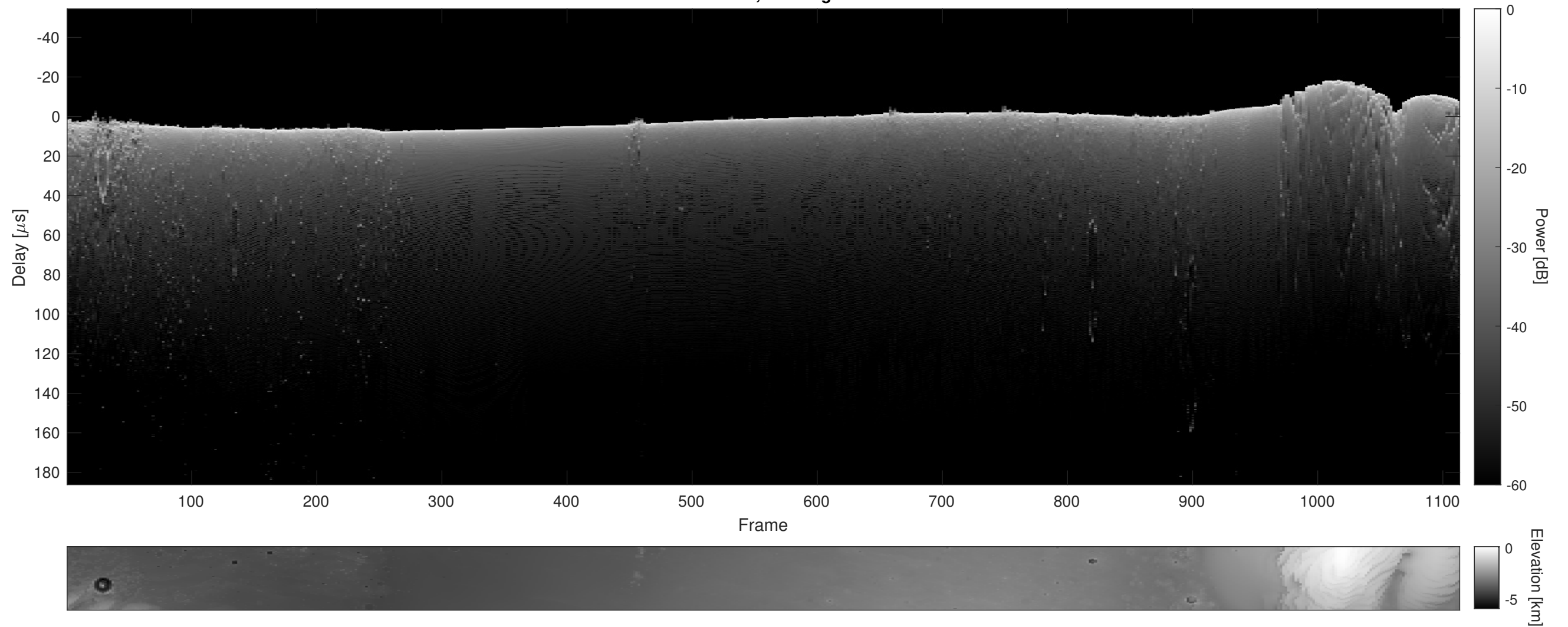
Orbit 12118, Cluttergram
