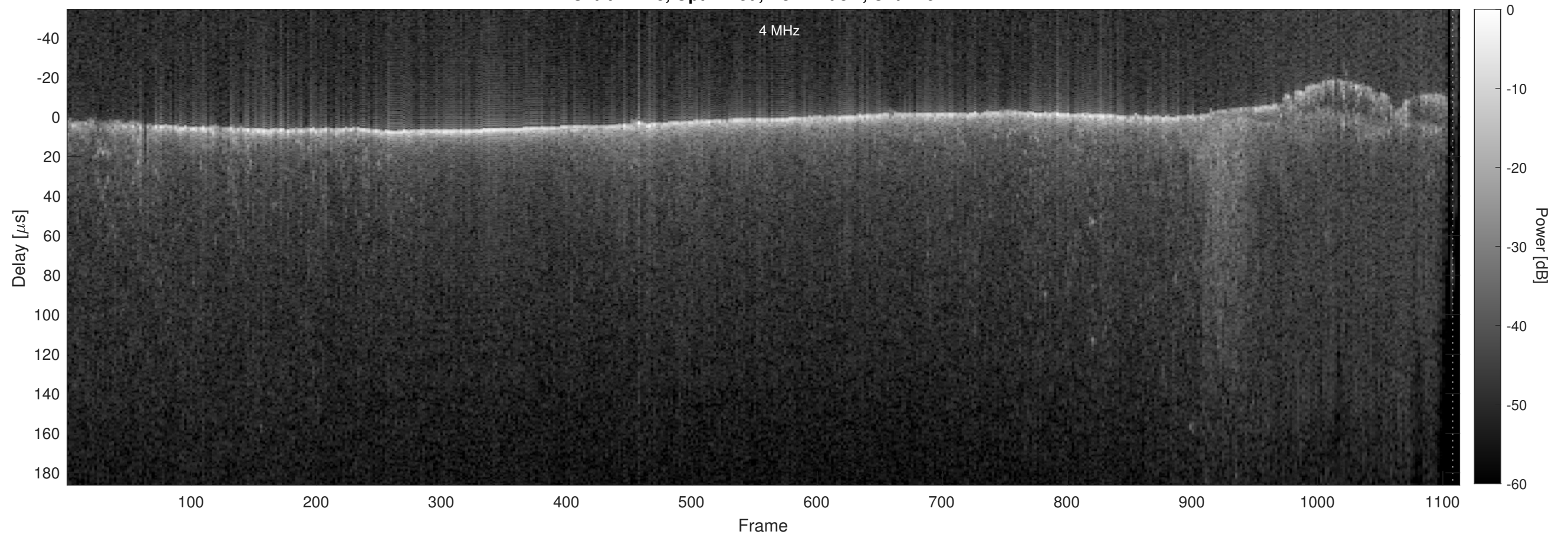
Orbit 12118, Optimized, No Window, Channel 2
