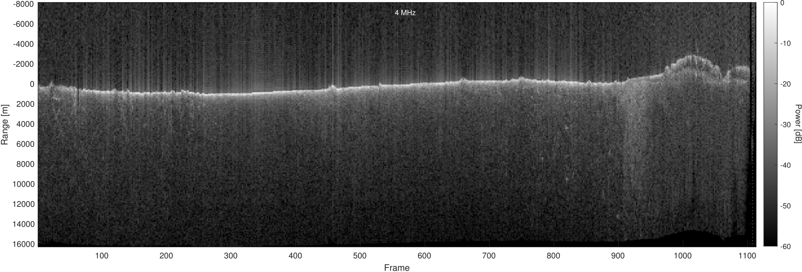
Orbit 12118, Optimized, No Window, Depth-Corrected, Channel 2
