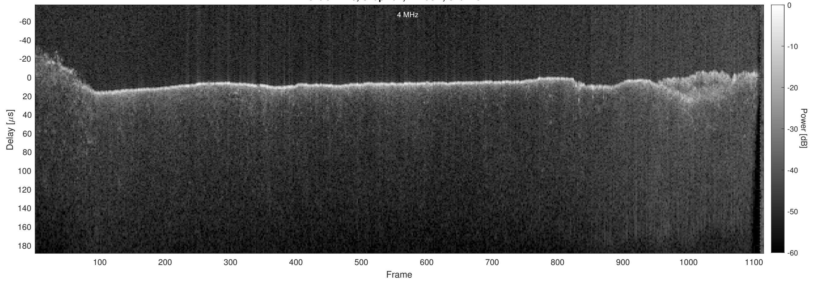
Orbit 12119, Chapman, Window, Channel 2
