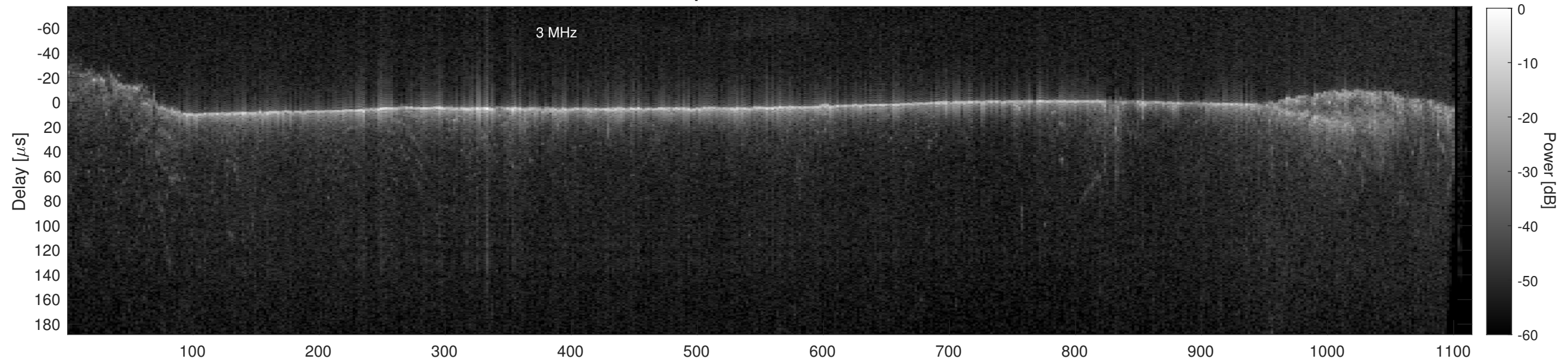
Orbit 12119, Cluttergram
