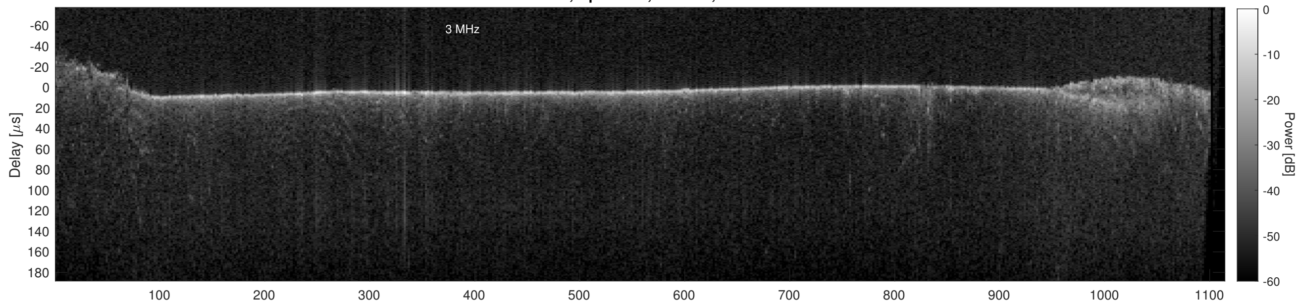
Orbit 12119, Cluttergram
