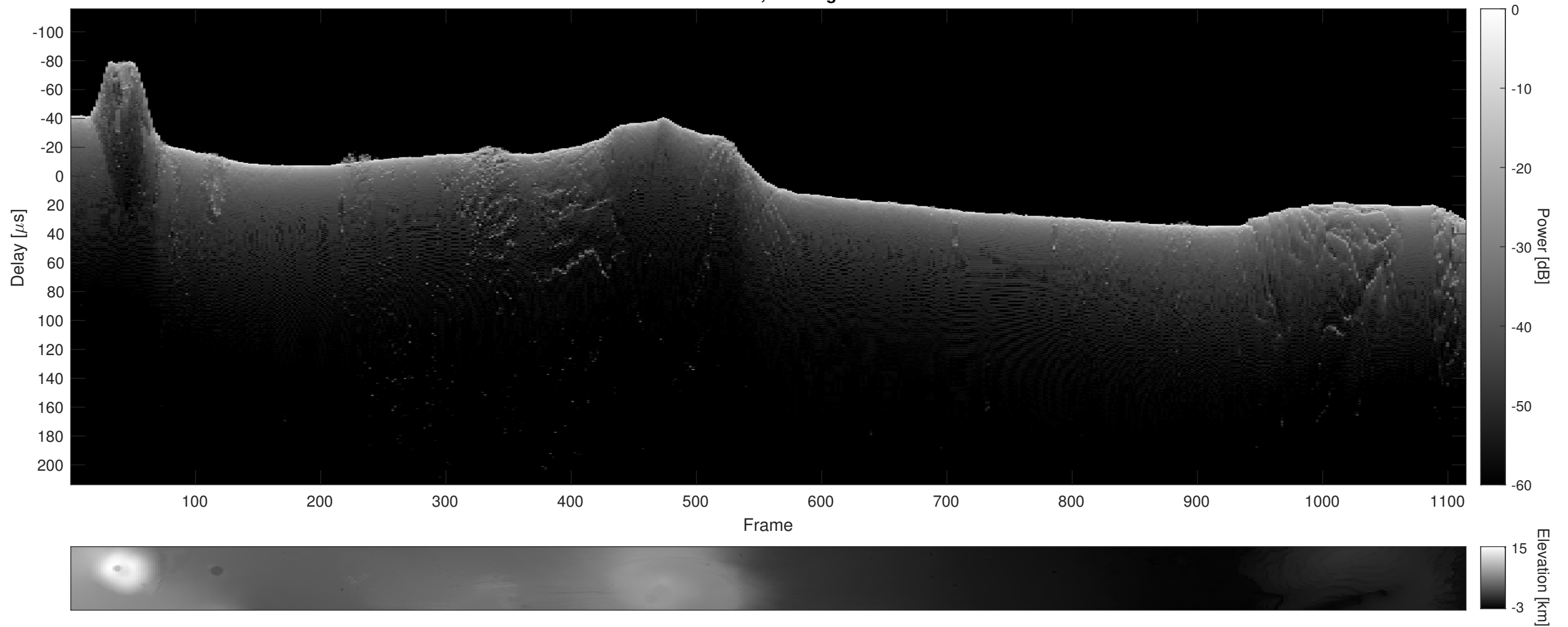
Orbit 12121, Cluttergram
