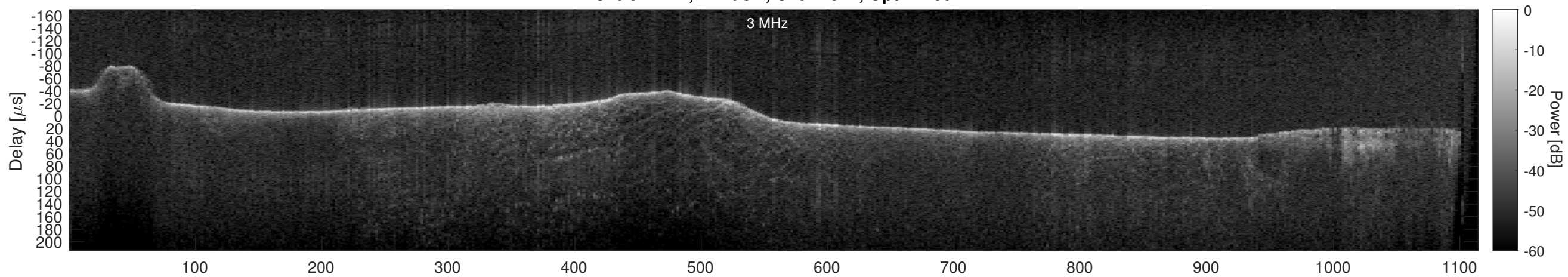
Orbit 12121, Cluttergram
