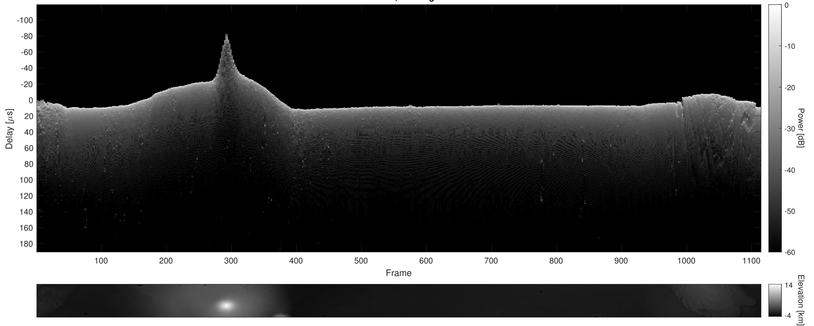
Orbit 12122, Cluttergram
