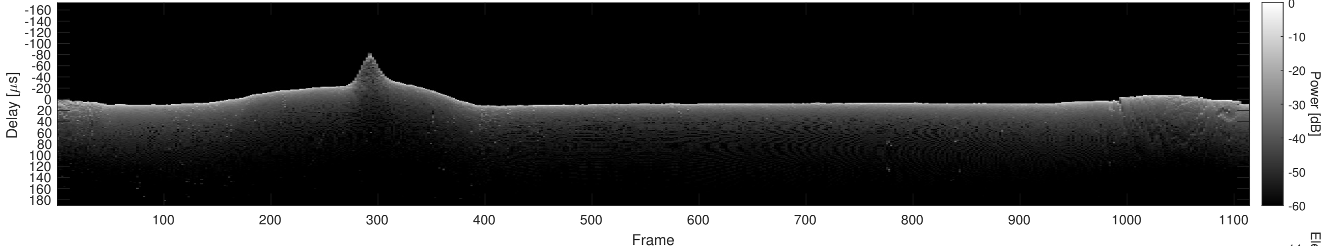
Orbit 12122, Cluttergram
