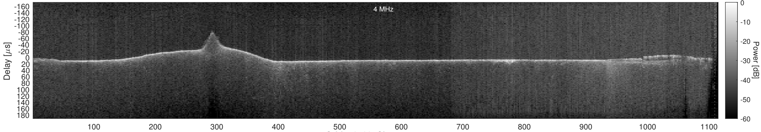
Orbit 12122, Cluttergram
