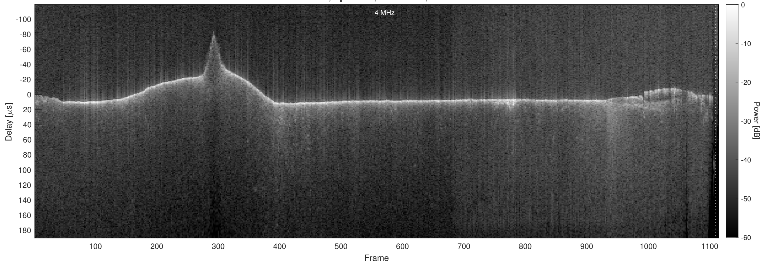
Orbit 12122, Optimized, No Window, Channel 2
