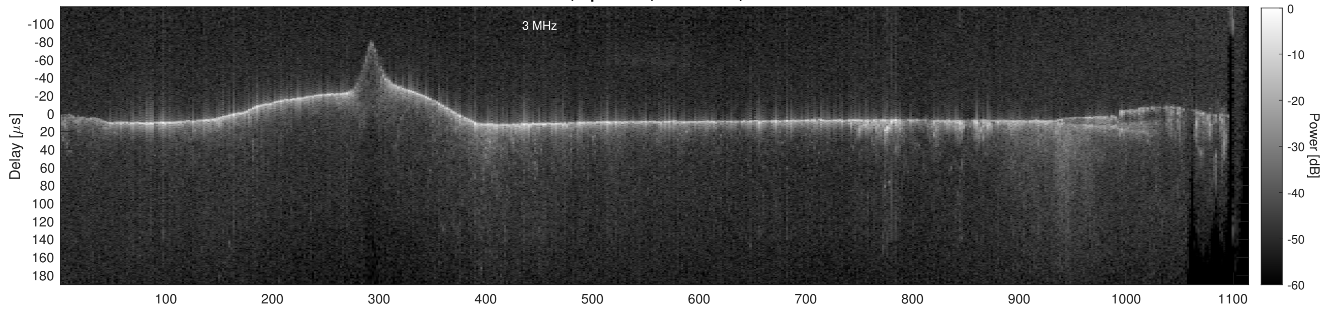
Orbit 12122, Cluttergram
