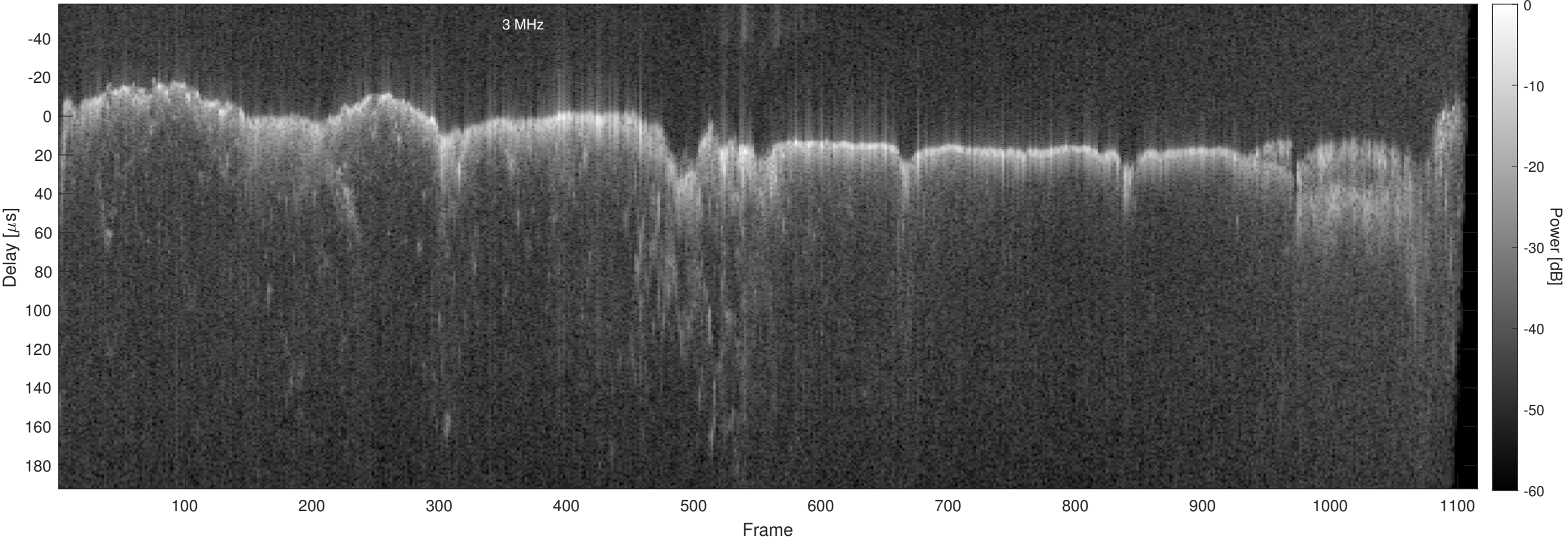
Orbit 12123, Chapman, No Window, Channel 2
