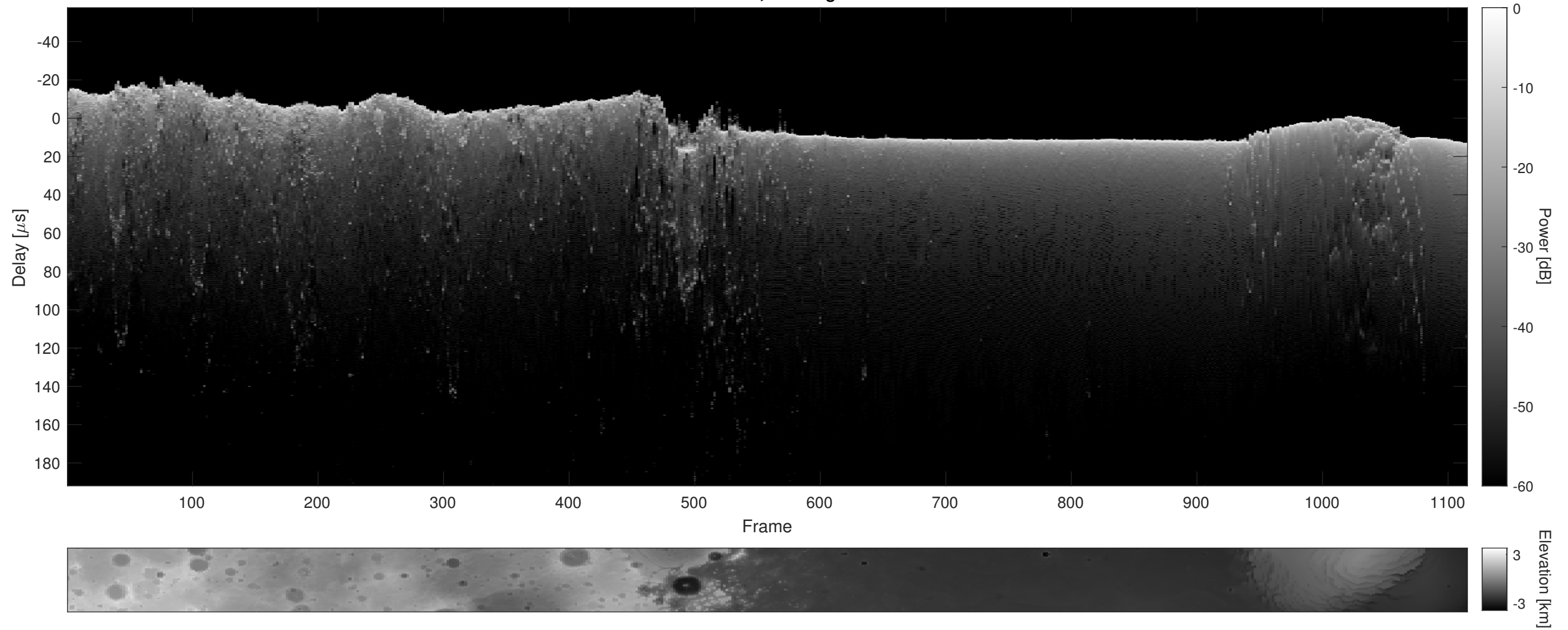
Orbit 12123, Cluttergram
