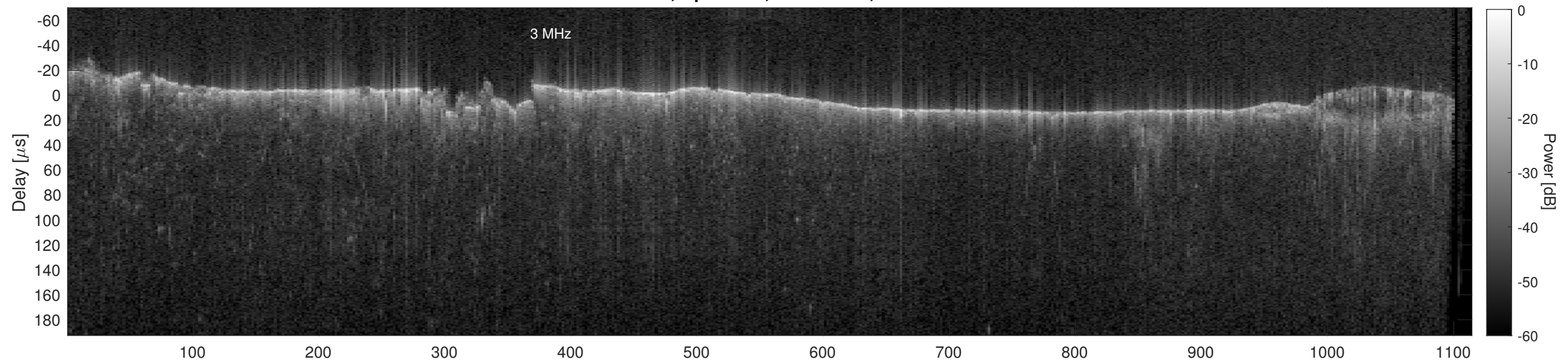
Orbit 12124, Cluttergram
