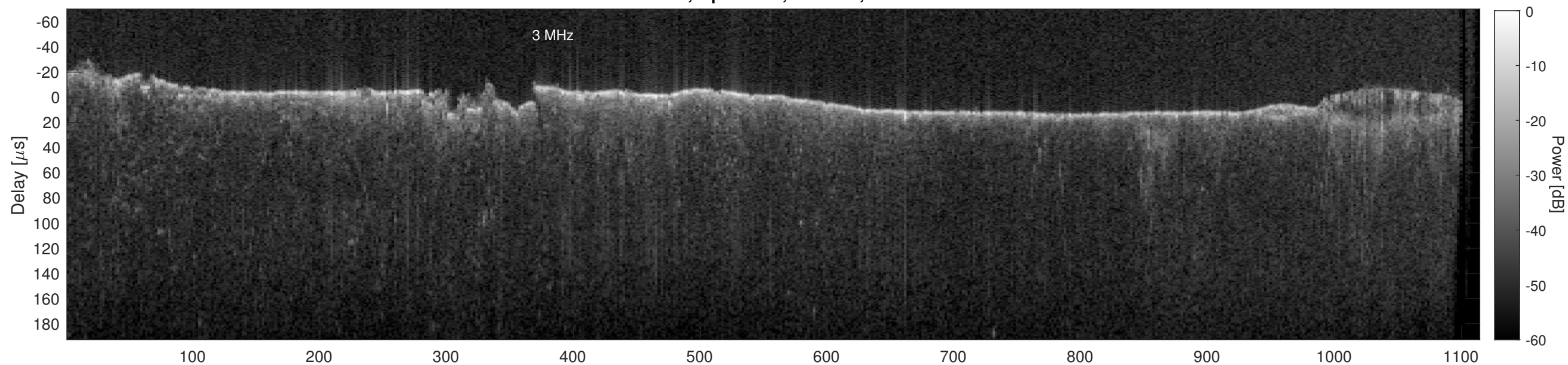
Orbit 12124, Cluttergram
