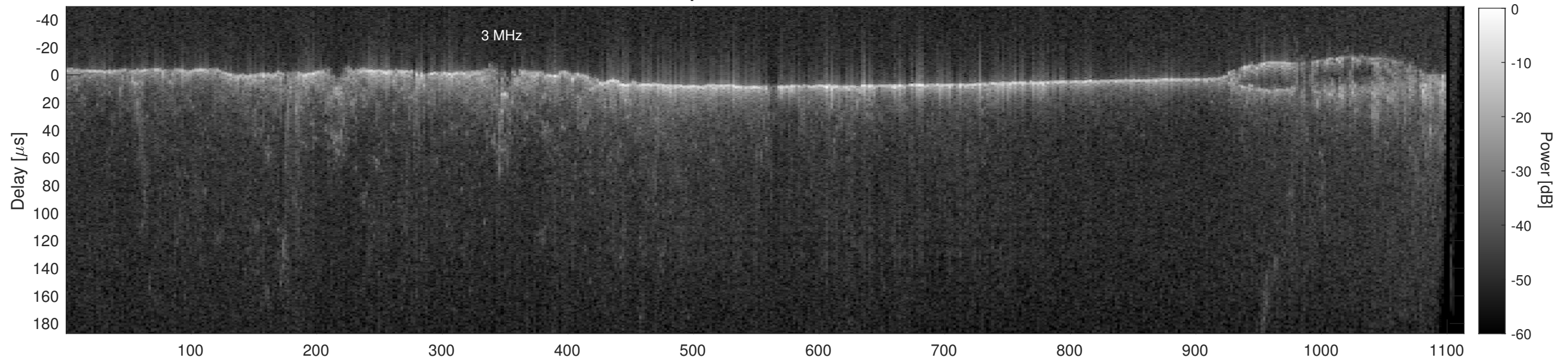
Orbit 12127, Cluttergram
