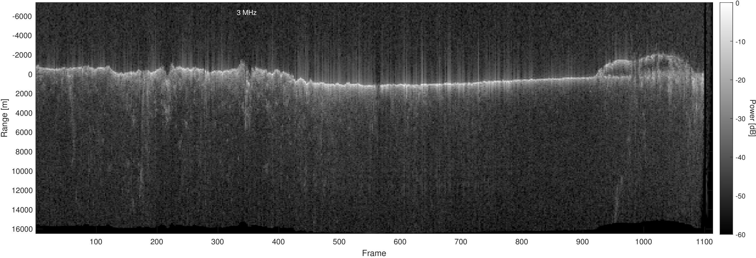
Orbit 12127, Optimized, No Window, Depth-Corrected, Channel 2
