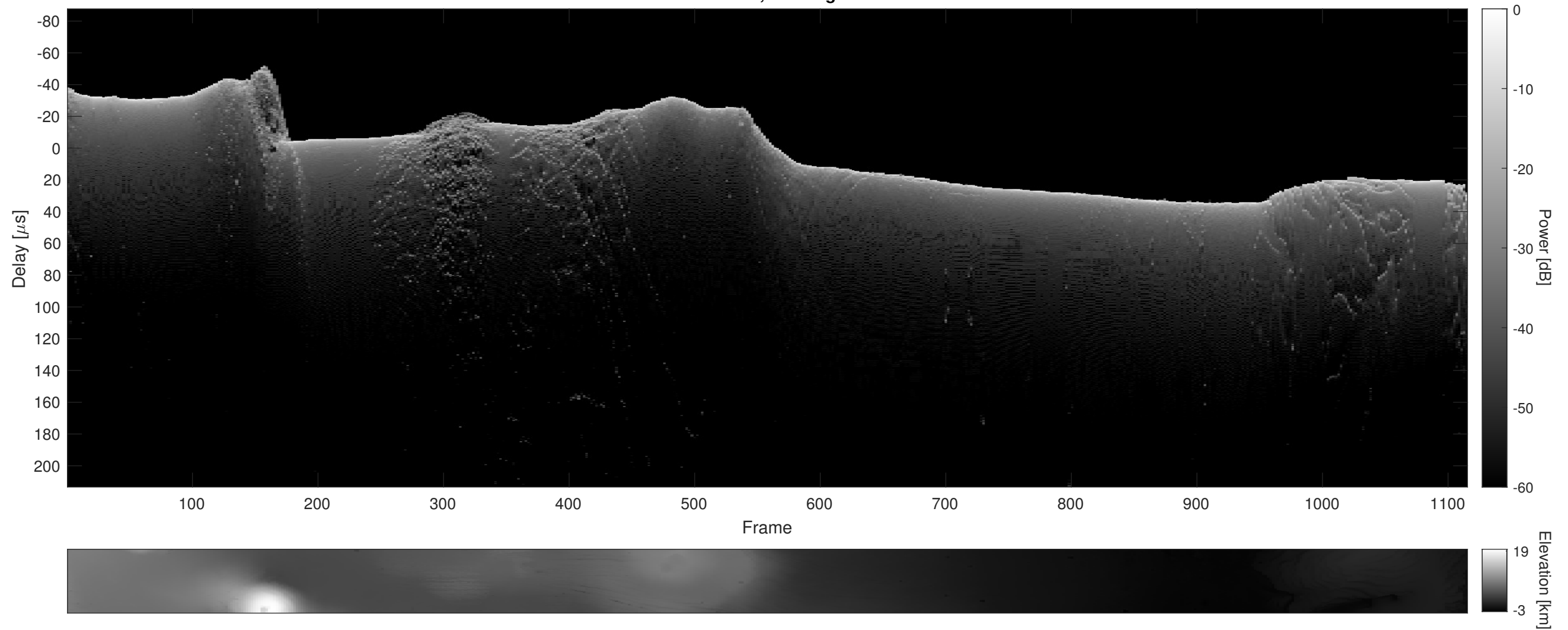
Orbit 12128, Cluttergram
