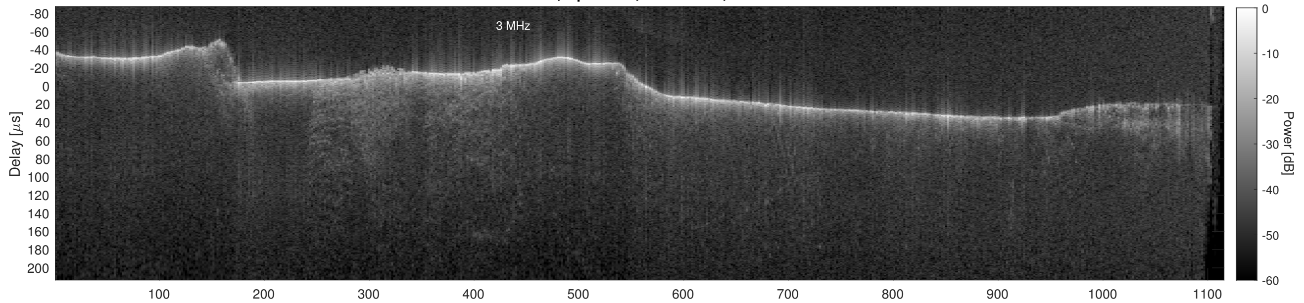
Orbit 12128, Cluttergram
