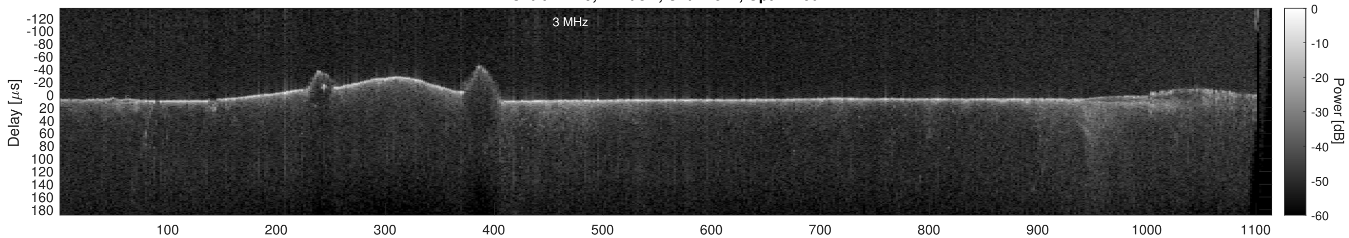
Orbit 12129, Cluttergram
