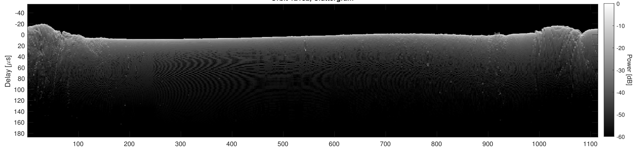
Orbit 12132, Cluttergram
