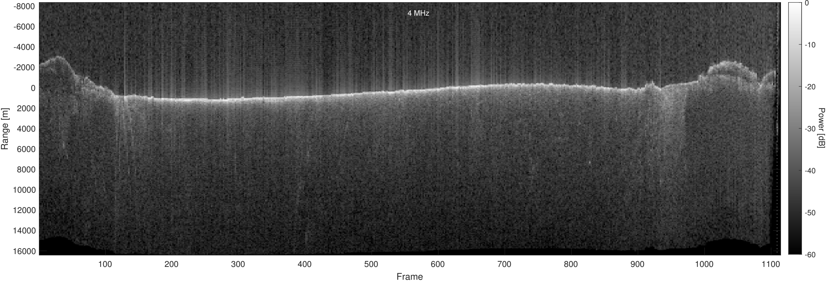
Orbit 12132, Optimized, No Window, Depth-Corrected, Channel 2
