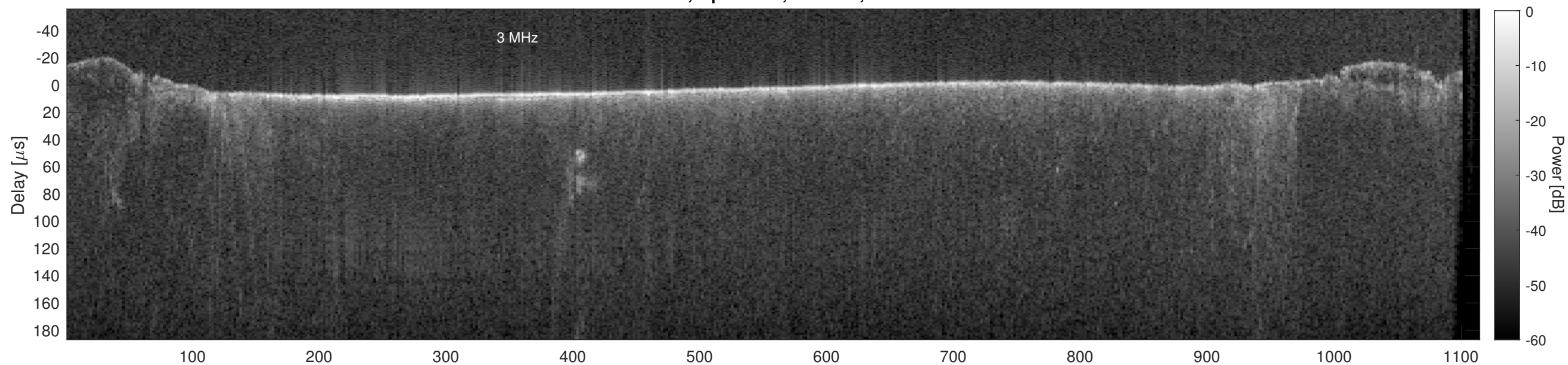
Orbit 12132, Cluttergram
