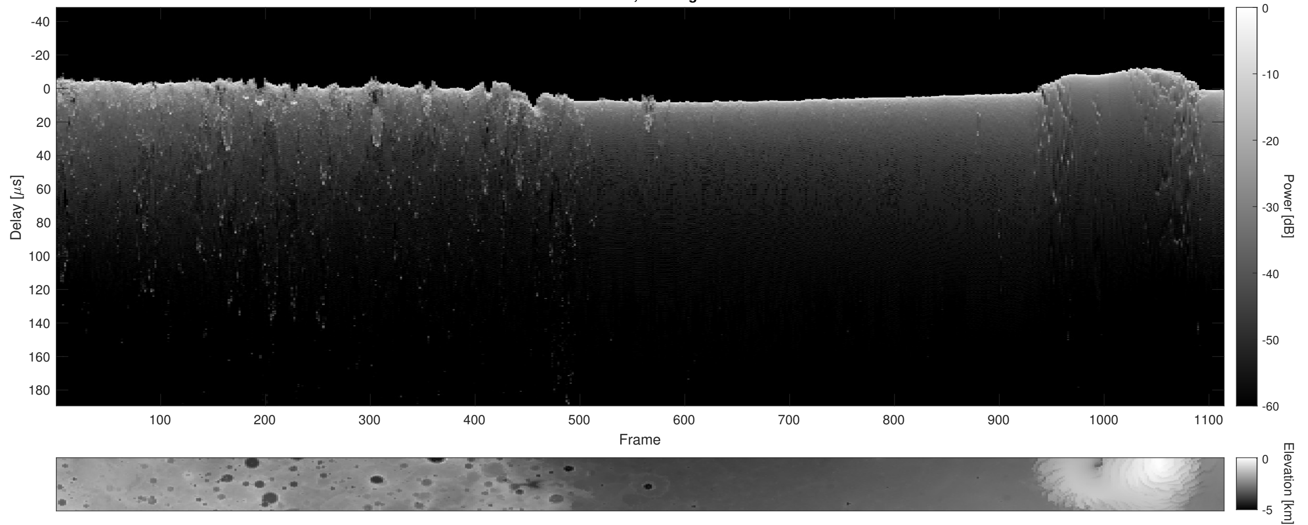
Orbit 12134, Cluttergram
