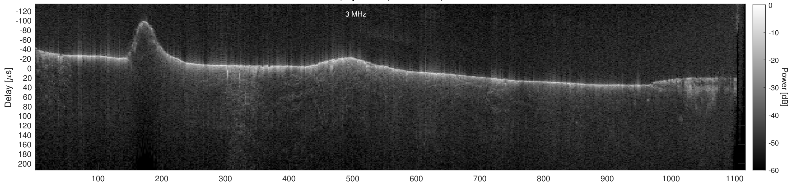
Orbit 12135, Cluttergram
