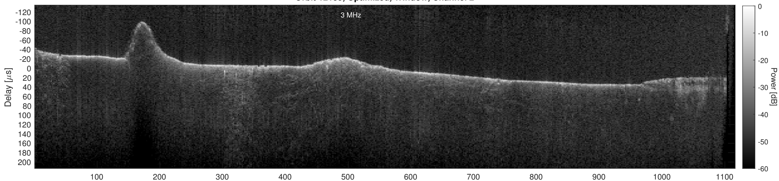
Orbit 12135, Cluttergram
