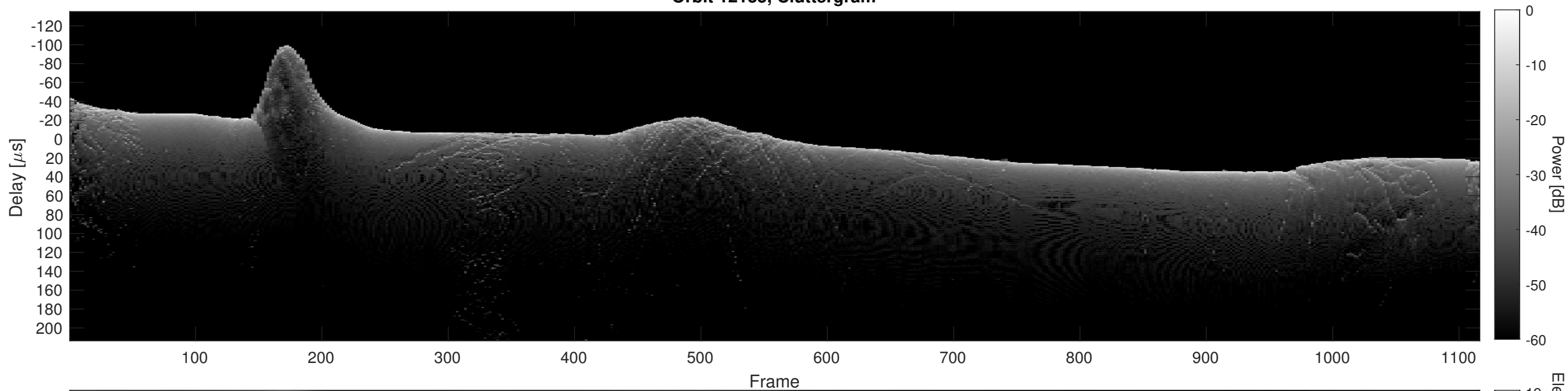
Orbit 12135, Cluttergram
