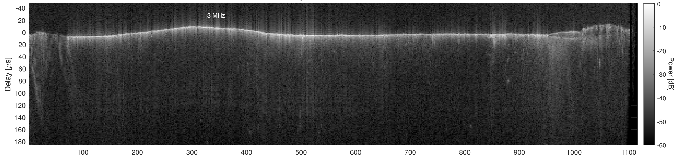
Orbit 12136, Cluttergram
