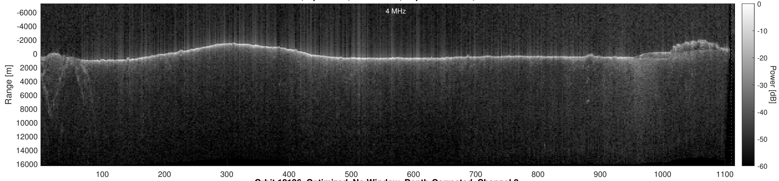
Orbit 12136, Optimized, No Window, Depth-Corrected, Channel 2
