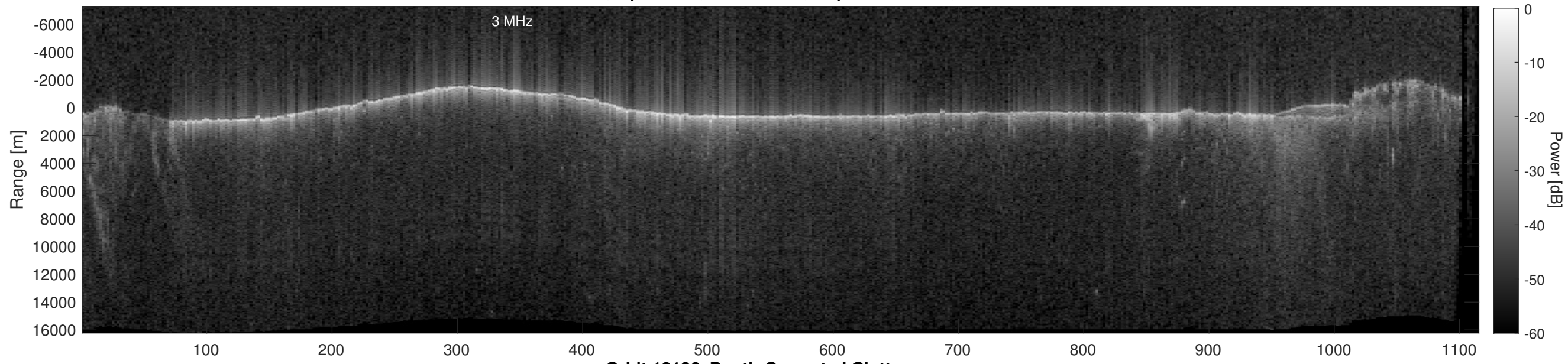
Orbit 12136, Depth-Corrected Cluttergram
