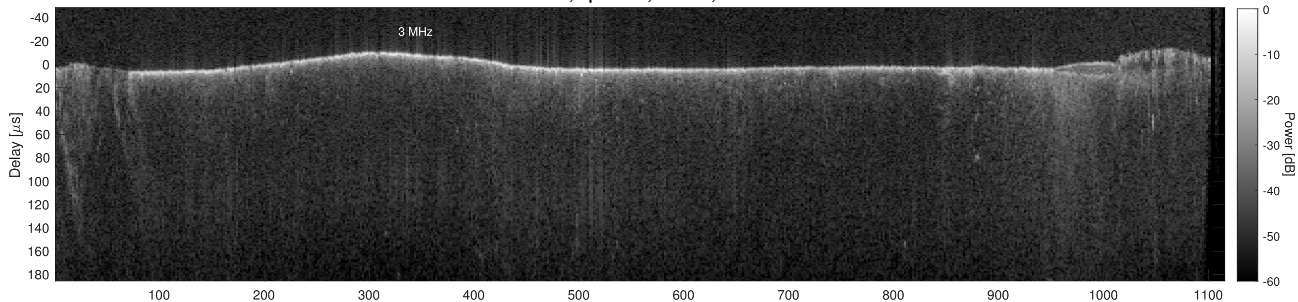
Orbit 12136, Cluttergram
