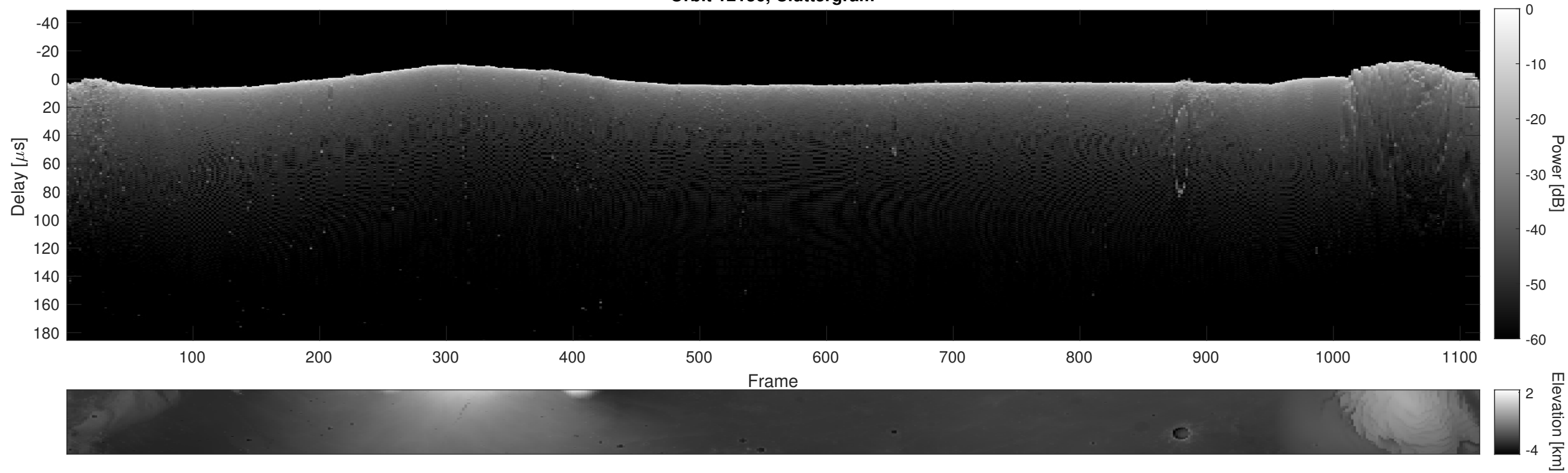
Orbit 12136, Cluttergram
