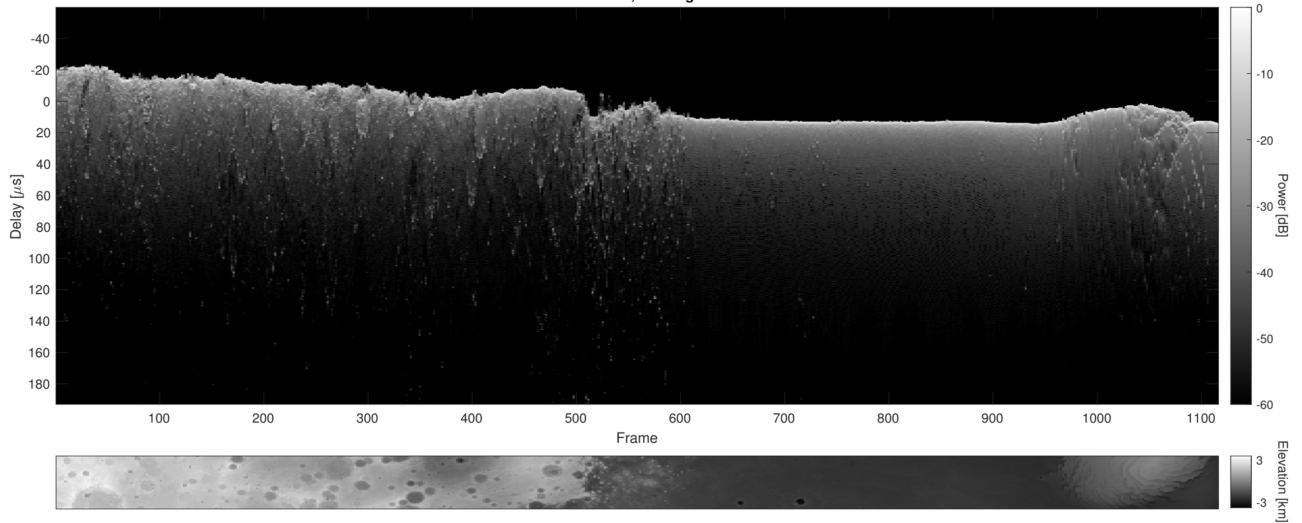
Orbit 12137, Cluttergram
