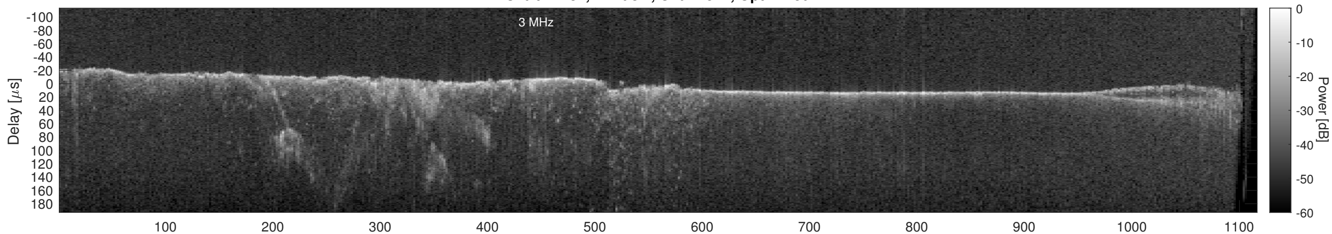
Orbit 12137, Cluttergram
